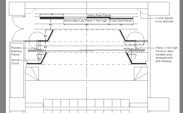
Revised STAGE PLAN
