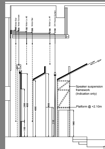
Revised STAGE SECTION
